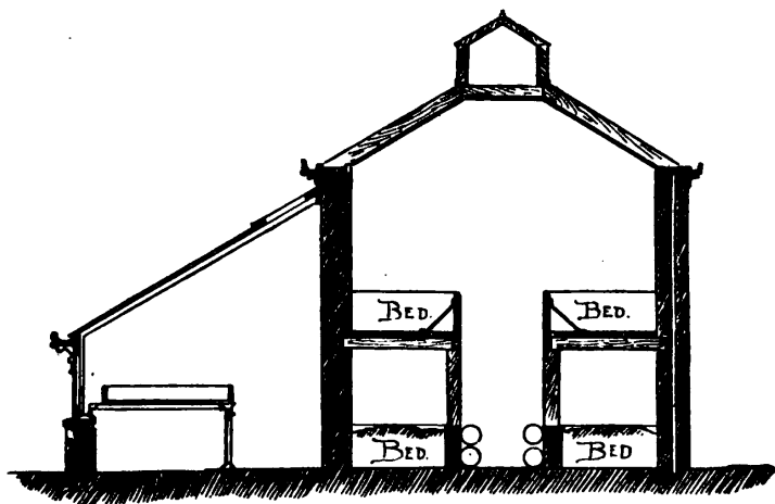
FIG. 8. SECTION OF MRS. C. J. OSBORNE'S MUSHROOM HOUSE.
