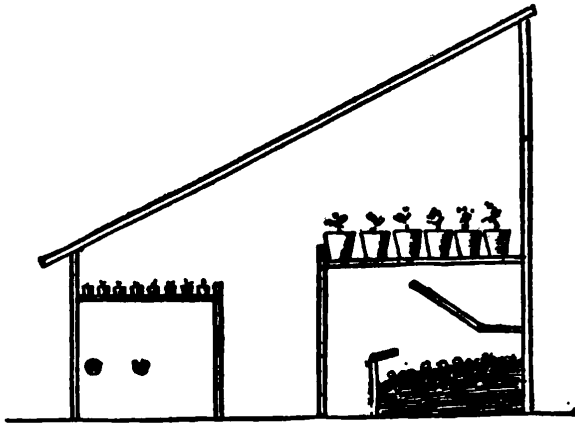
FIG. 11. BOXED MUSHROOM BED UNDER GREENHOUSE BENCH.
