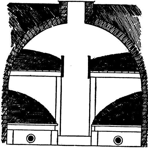
FIG. 3. CROSS-SECTION OF THE DOSORIS MUSHROOM CELLAR.
