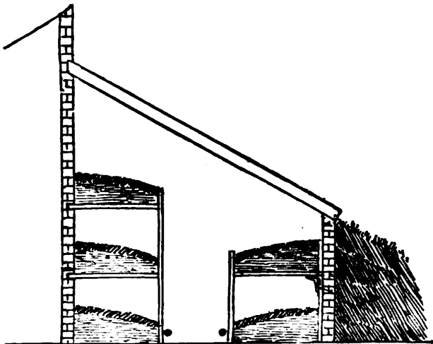
FIG. 7. MUSHROOM HOUSE BUILT AGAINST A NORTH-FACING WALL.
