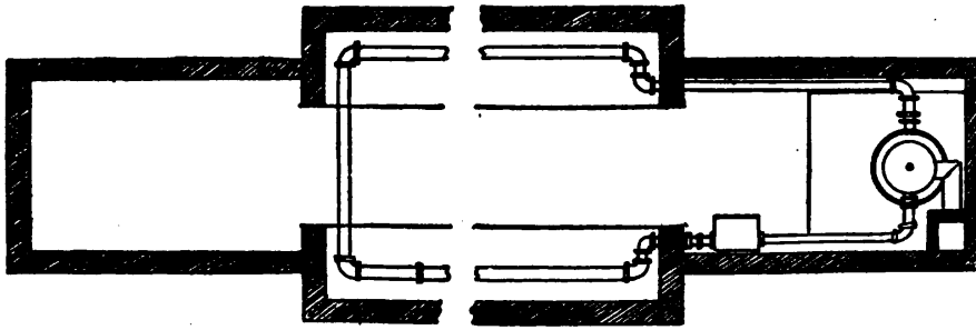
FIG. 4. GROUND PLAN OP THE DOSORIS CELLAR.
