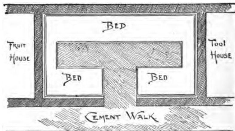
FIG. 9. GROUND PLAN OF MRS. OSBORNE'S MUSBROOM HOUSE.
